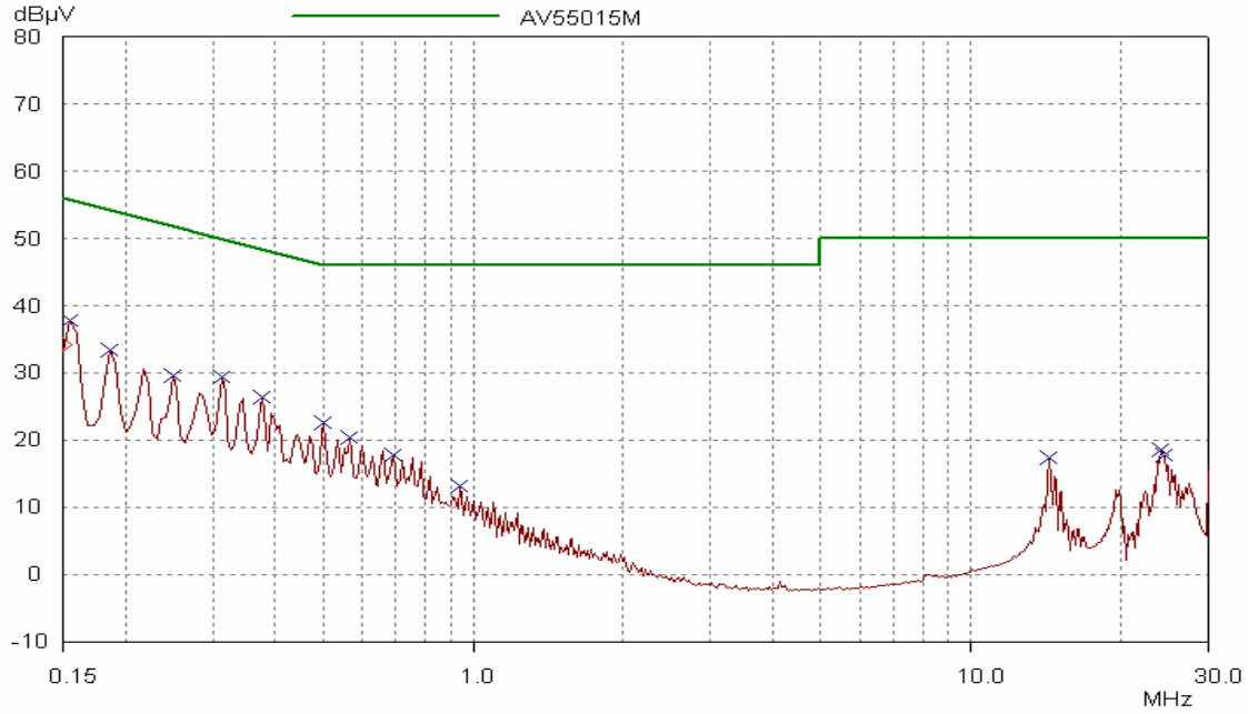
Plot 1b - Q117CAN1- Average Measurement - Neutral Port
