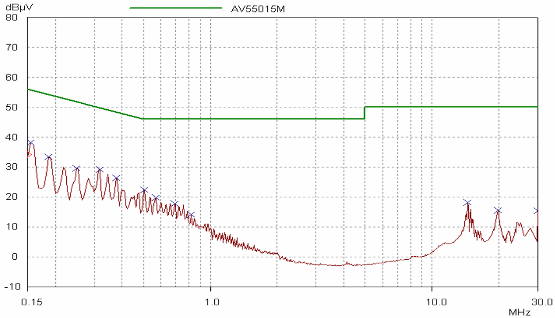
Plot 1a - Q117CAL1 - Average Measurement - Live Port
