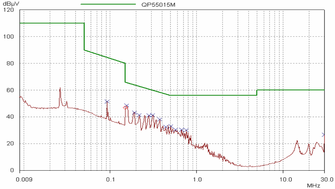
Plot 1c - Q117CQL1 - Quasi Peak Measurement - Live Port
