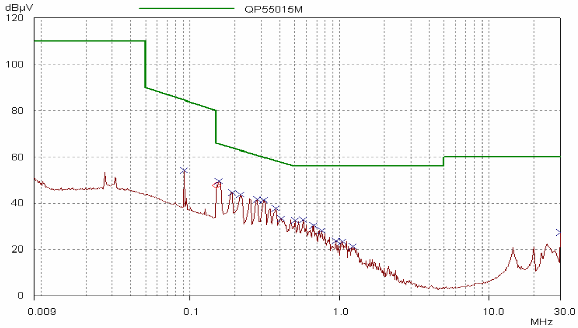
Plot 1d - Q117CQN1 - Quasi Peak Measurement - Neutral Port
